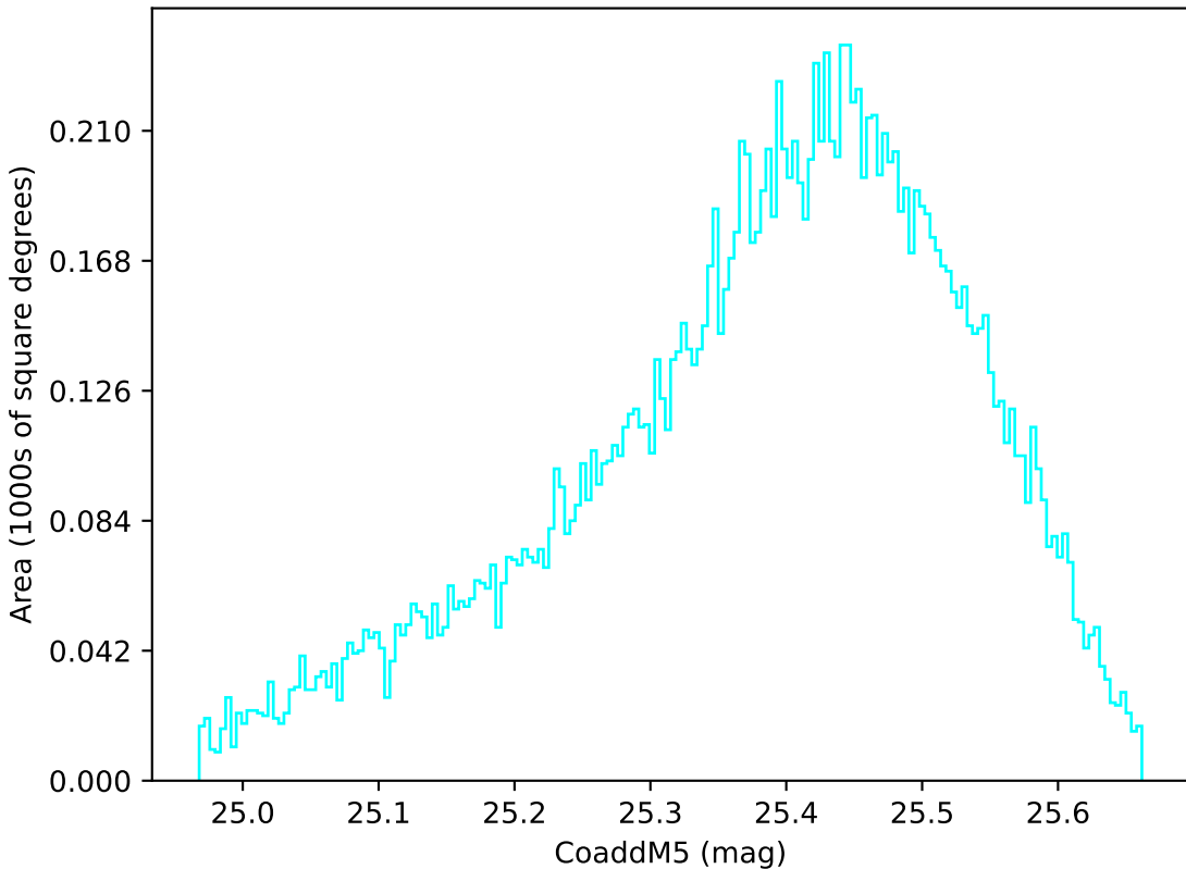
no_high_blob_v3.3_10yrs WFD u band: CoaddM5
