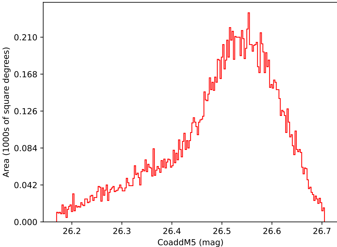
no_high_blob_v3.3_10yrs WFD i band: CoaddM5
