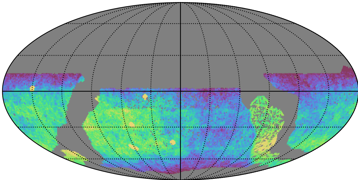
no_high_blob_v3.3_10yrs WFD g band: CoaddM5
