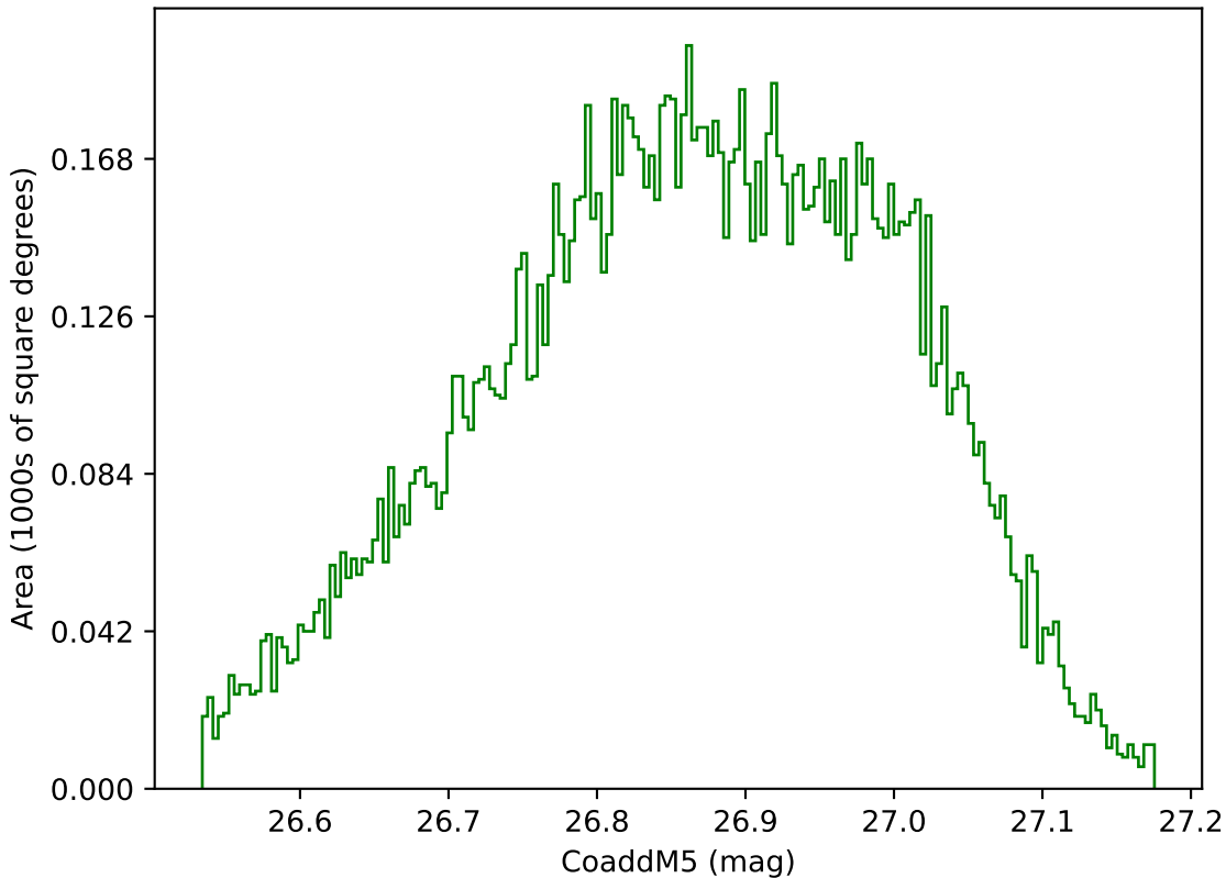
no_high_blob_v3.3_10yrs WFD g band: CoaddM5
