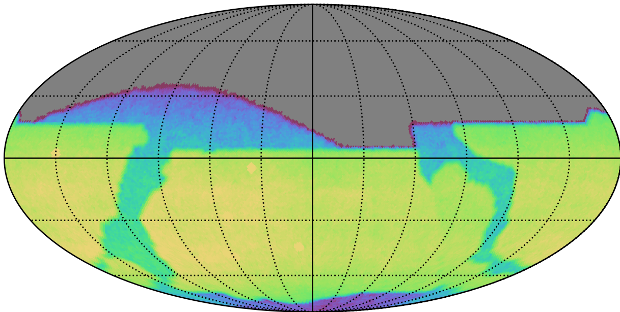
no_high_blob_v3.3_10yrs All sky z band: CoaddM5
