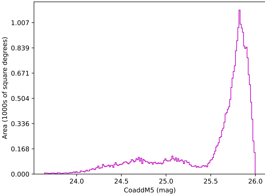
no_high_blob_v3.3_10yrs All sky z band: CoaddM5
