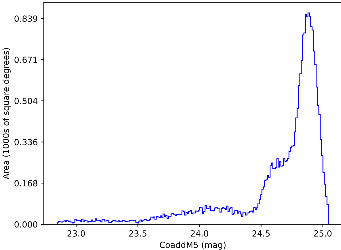
no_high_blob_v3.3_10yrs All sky y band: CoaddM5
