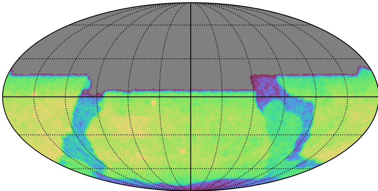
no_high_blob_v3.3_10yrs All sky u band: CoaddM5
