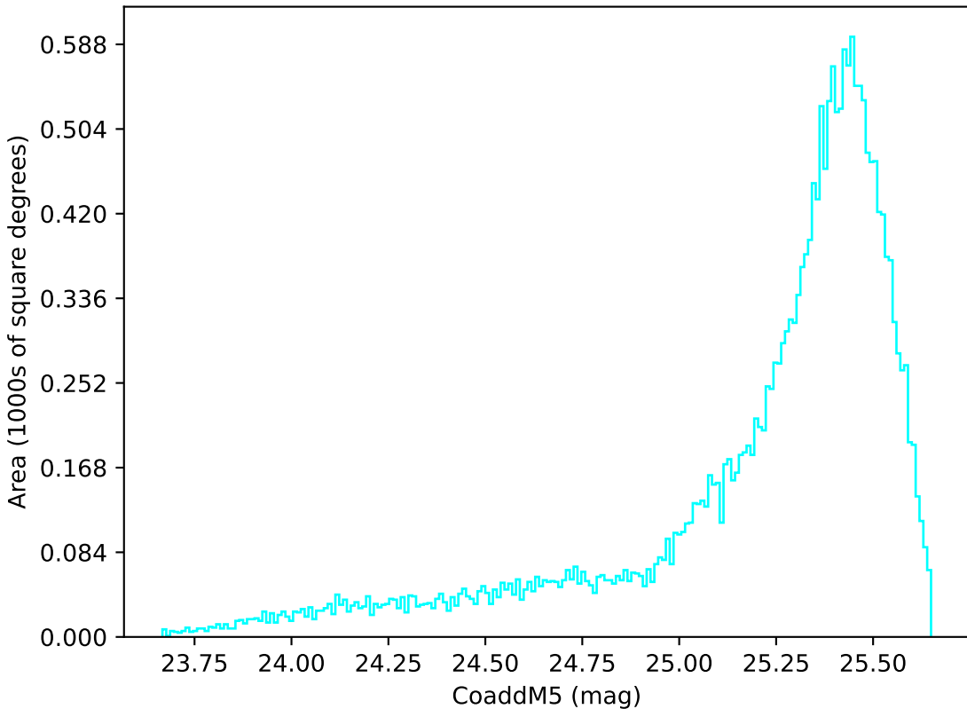
no_high_blob_v3.3_10yrs All sky u band: CoaddM5
