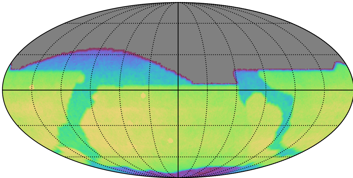
no_high_blob_v3.3_10yrs All sky r band: CoaddM5
