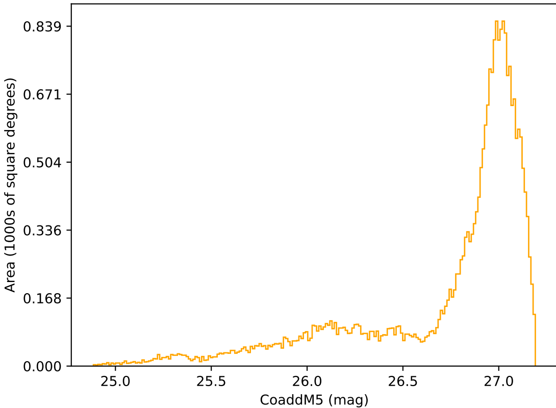
no_high_blob_v3.3_10yrs All sky r band: CoaddM5
