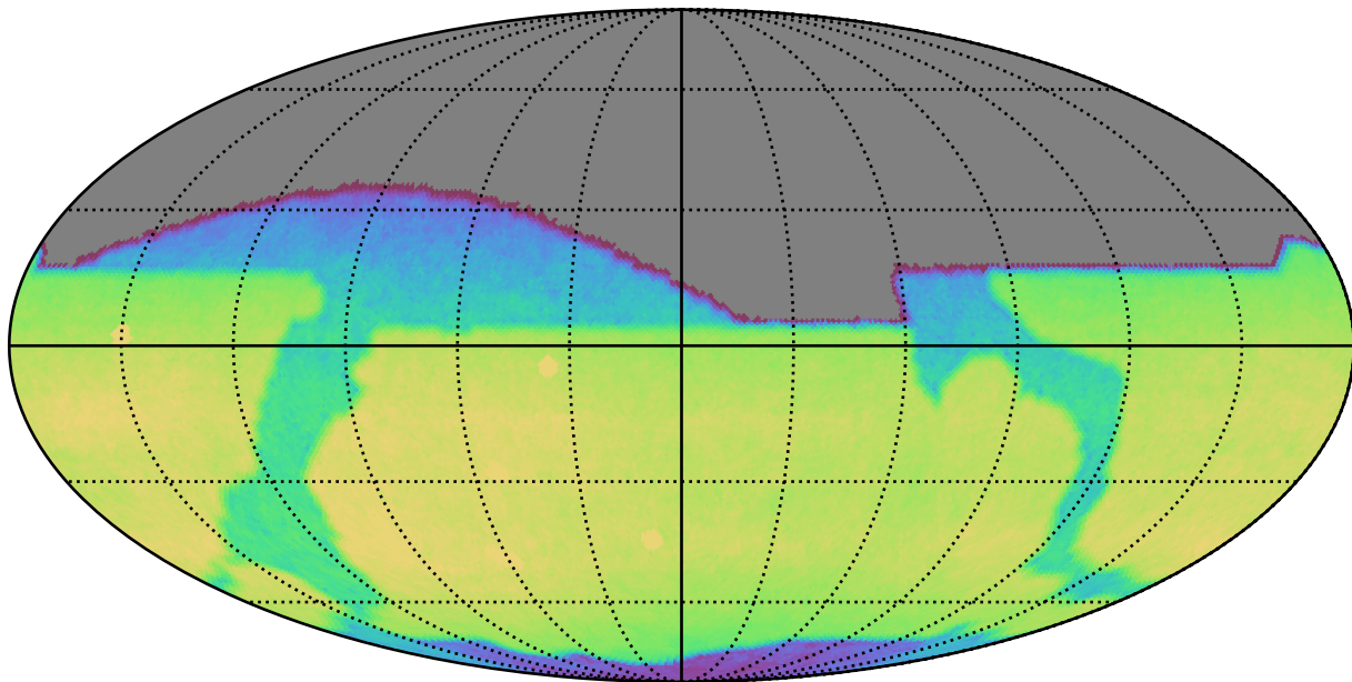
no_high_blob_v3.3_10yrs All sky i band: CoaddM5
