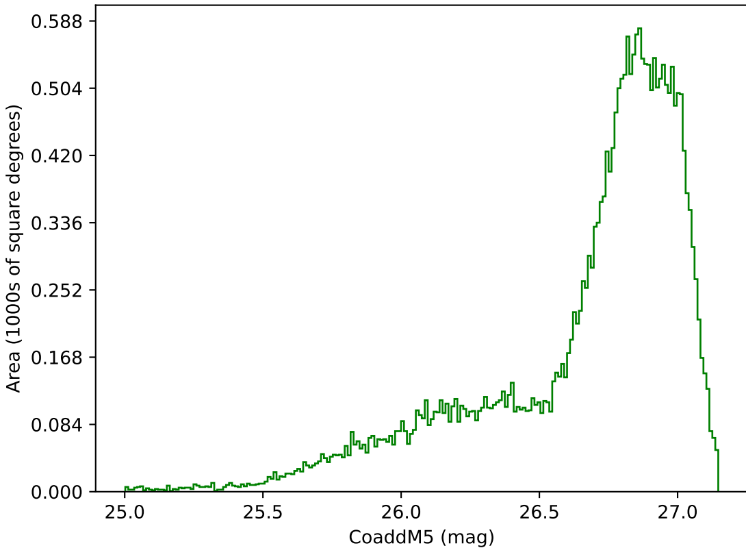
no_high_blob_v3.3_10yrs All sky g band: CoaddM5
