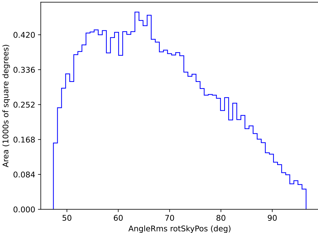
no_high_blob_v3.3_10yrs WFD z band: AngleRms rotSkyPos
