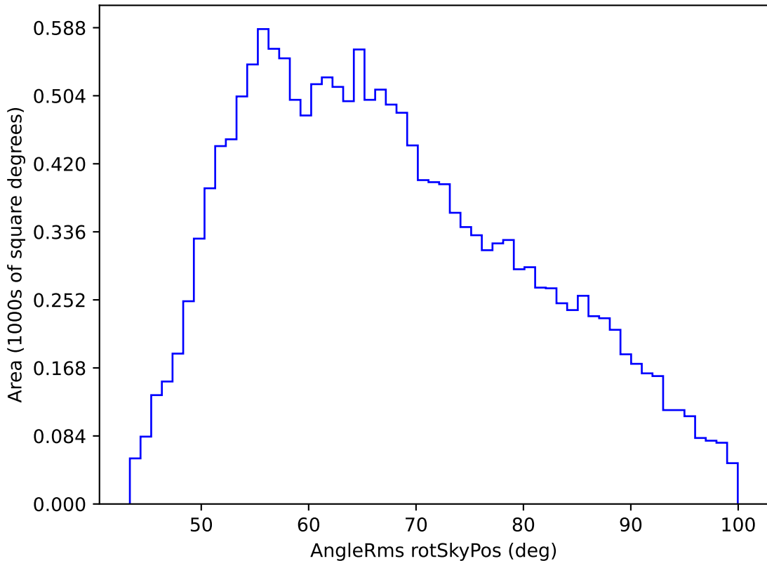
no_high_blob_v3.3_10yrs WFD u band: AngleRms rotSkyPos
