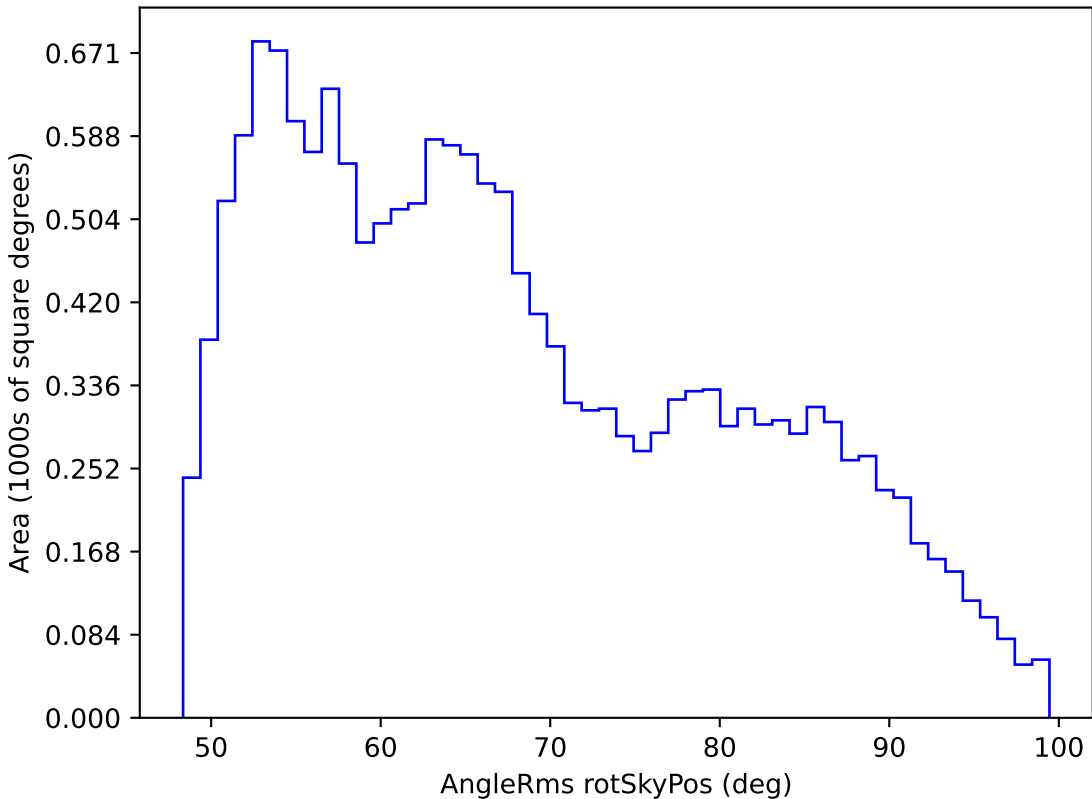
no_high_blob_v3.3_10yrs WFD r band: AngleRms rotSkyPos
