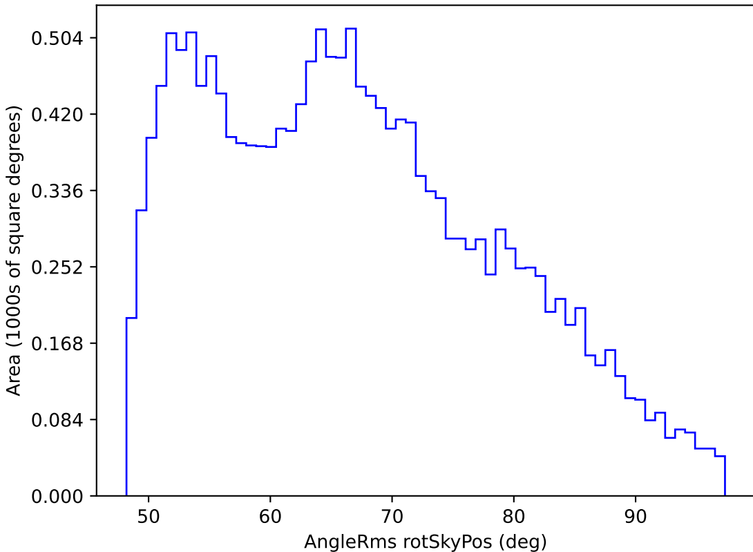
no_high_blob_v3.3_10yrs WFD i band: AngleRms rotSkyPos
