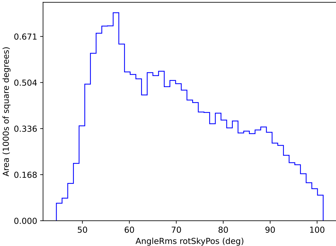
no_high_blob_v3.3_10yrs WFD g band: AngleRms rotSkyPos
