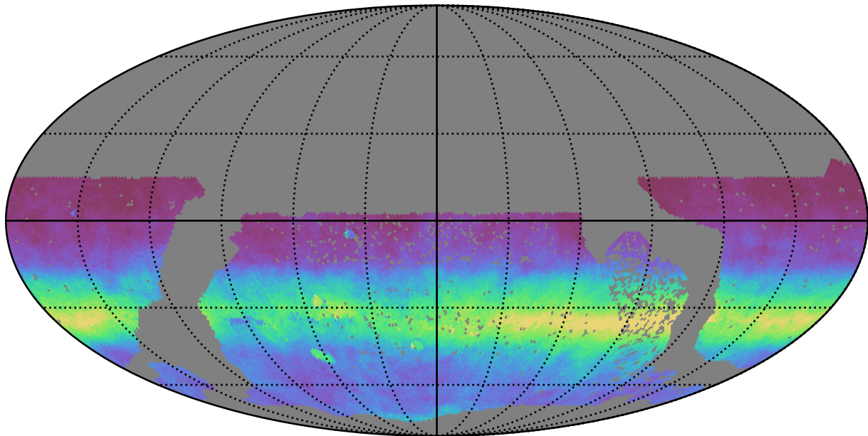
no_high_blob_v3.3_10yrs WFD all bands: AngleRms rotSkyPos
