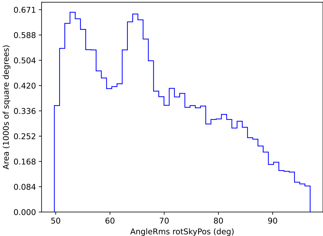
no_high_blob_v3.3_10yrs WFD all bands: AngleRms rotSkyPos
