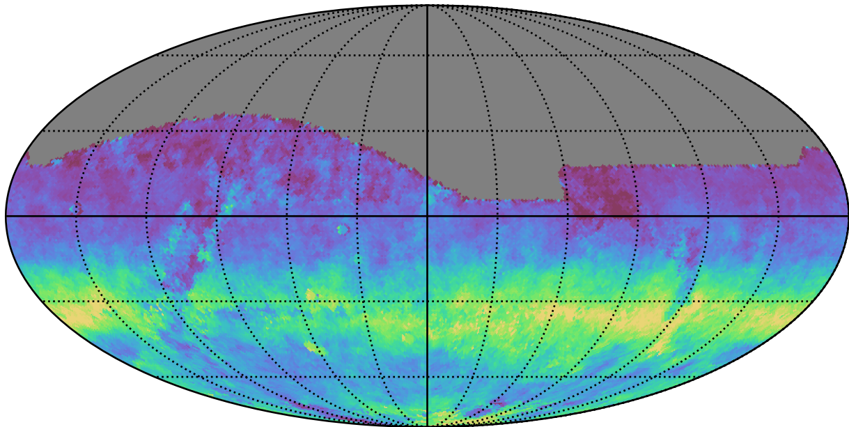
no_high_blob_v3.3_10yrs All sky z band: AngleRms rotSkyPos
