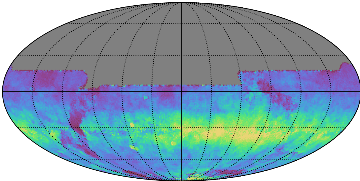
no_high_blob_v3.3_10yrs All sky y band: AngleRms rotSkyPos
