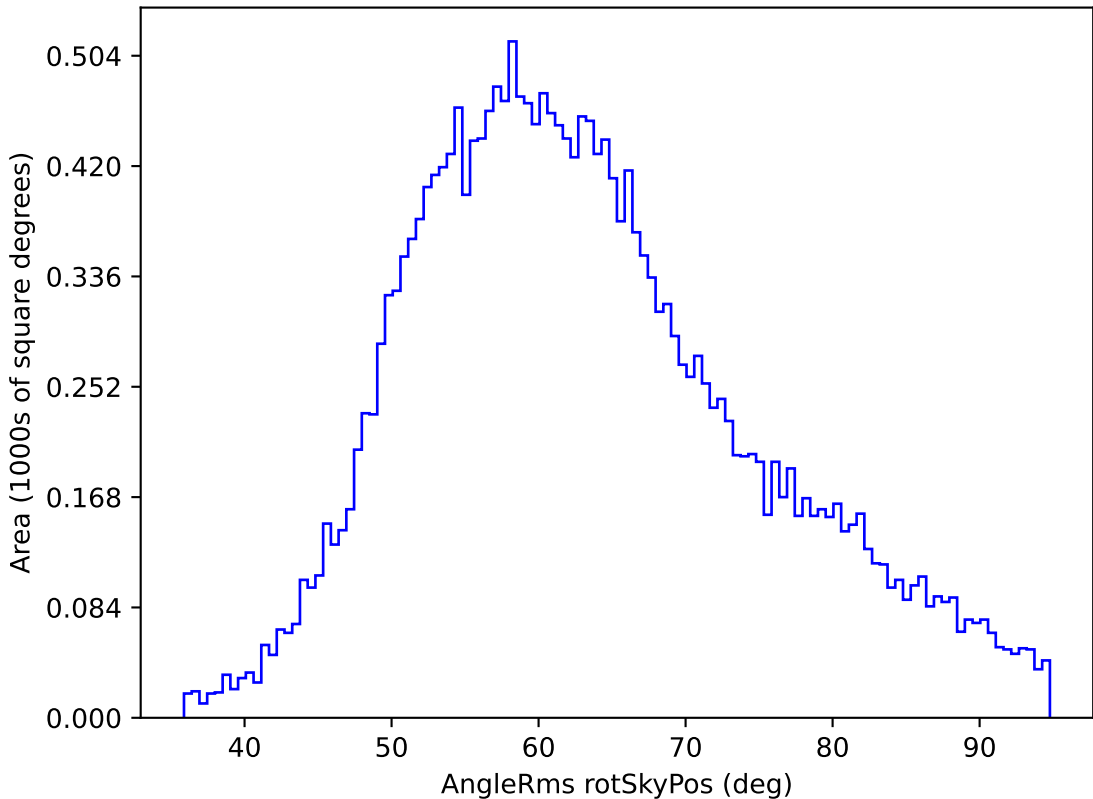
no_high_blob_v3.3_10yrs All sky y band: AngleRms rotSkyPos
