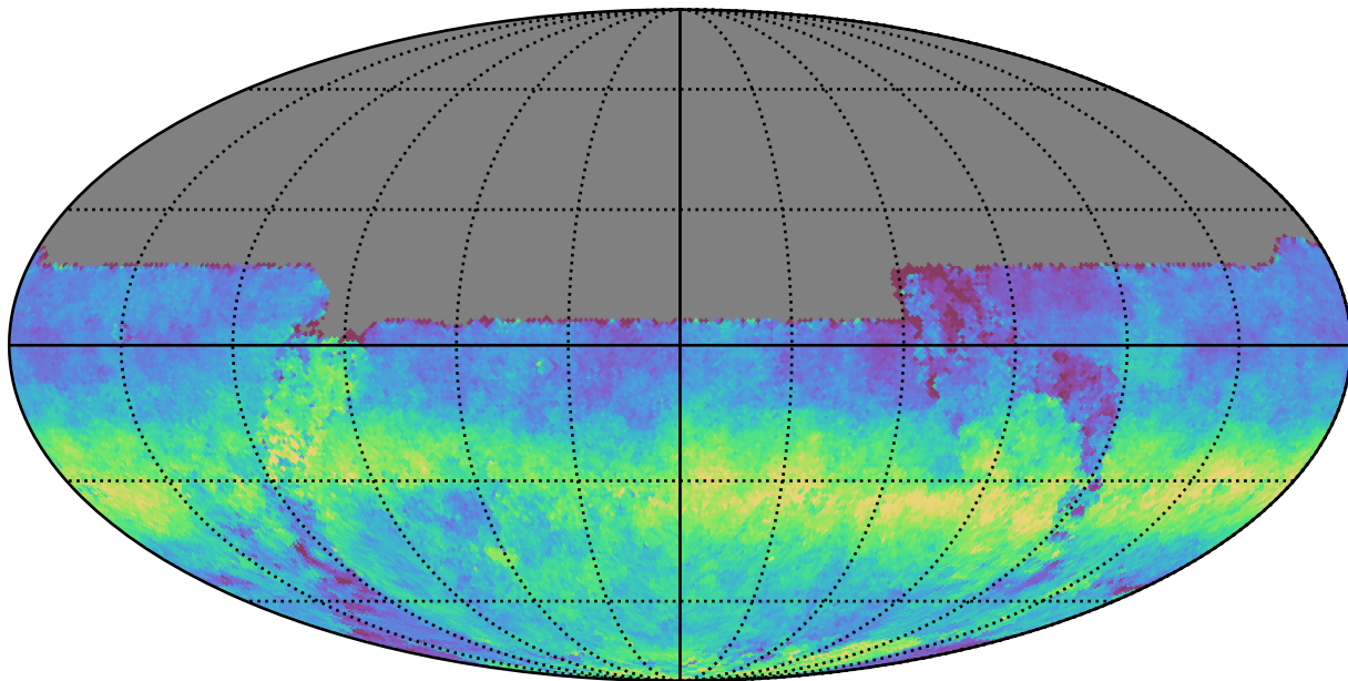
no_high_blob_v3.3_10yrs All sky u band: AngleRms rotSkyPos
