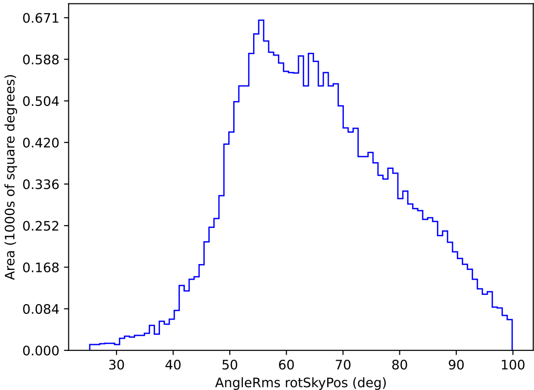
no_high_blob_v3.3_10yrs All sky u band: AngleRms rotSkyPos
