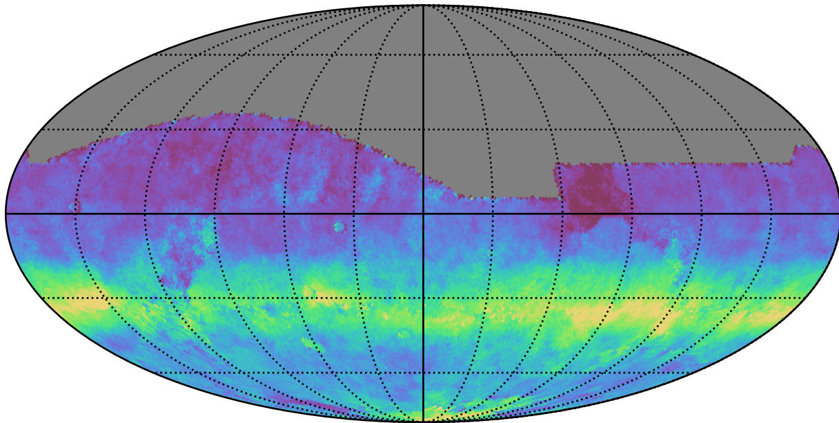
no_high_blob_v3.3_10yrs All sky i band: AngleRms rotSkyPos
