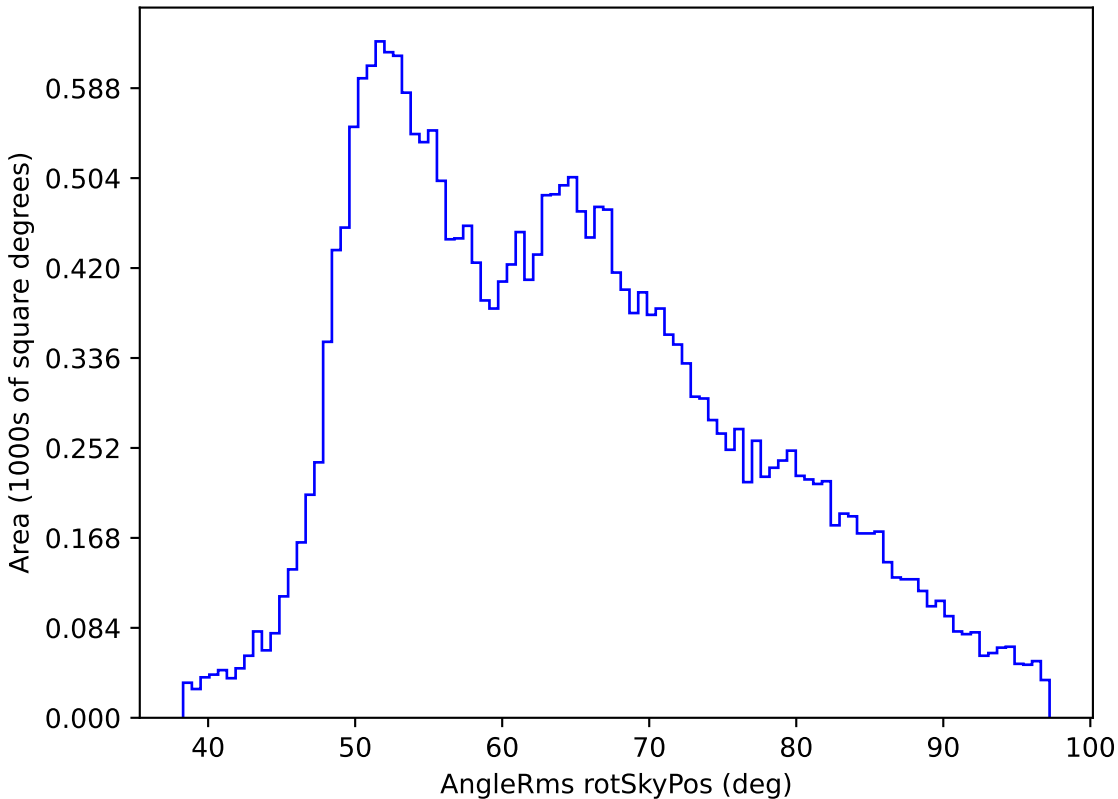
no_high_blob_v3.3_10yrs All sky i band: AngleRms rotSkyPos
