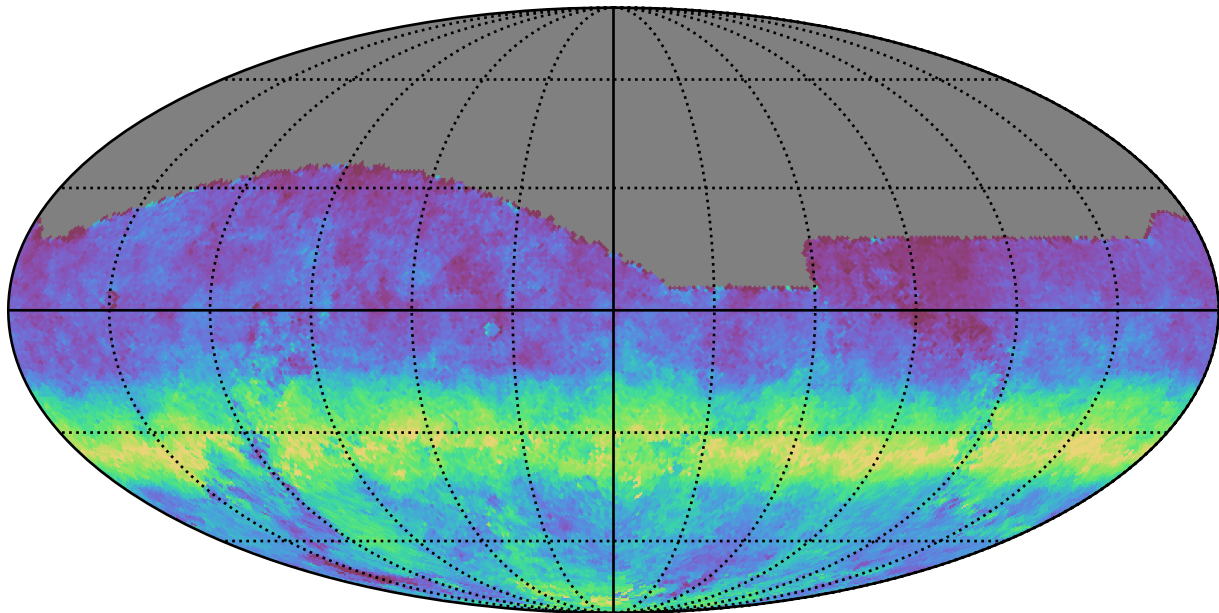
no_high_blob_v3.3_10yrs All sky g band: AngleRms rotSkyPos
