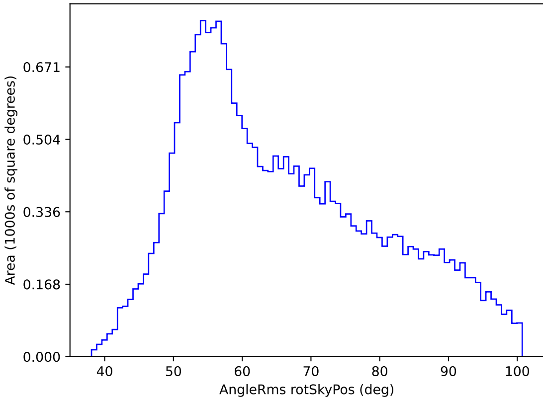
no_high_blob_v3.3_10yrs All sky g band: AngleRms rotSkyPos
