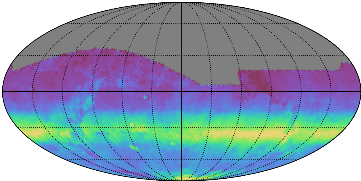
no_high_blob_v3.3_10yrs All sky all bands: AngleRms rotSkyPos
