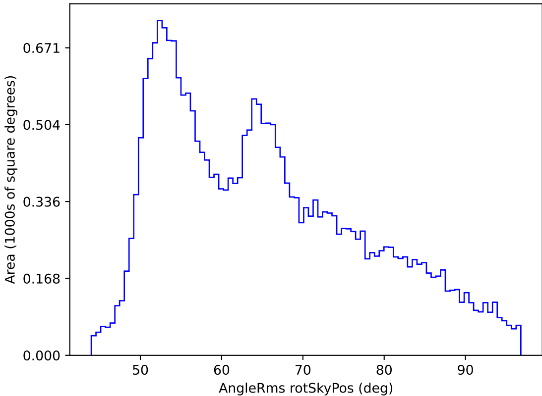
no_high_blob_v3.3_10yrs All sky all bands: AngleRms rotSkyPos
