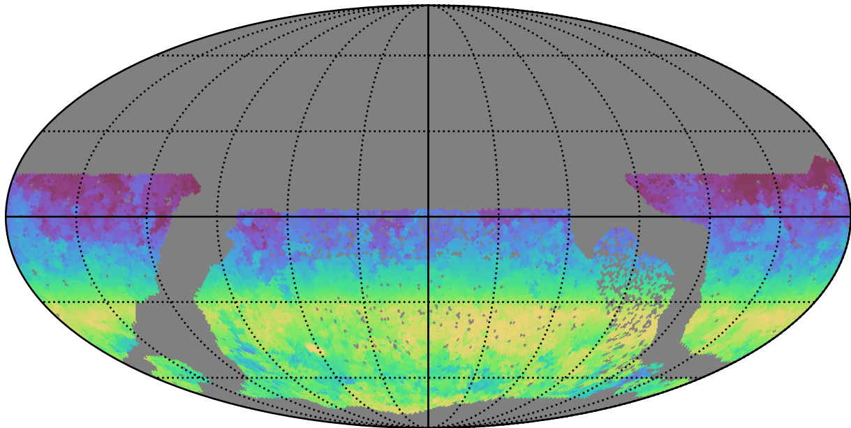
no_high_blob_v3.3_10yrs WFD z band: AngleRange rotSkyPos
