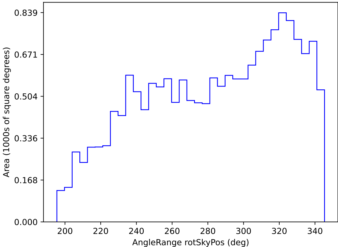
no_high_blob_v3.3_10yrs WFD z band: AngleRange rotSkyPos
