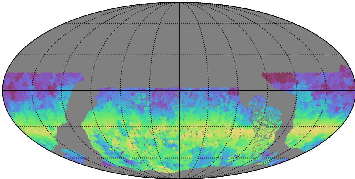
no_high_blob_v3.3_10yrs WFD u band: AngleRange rotSkyPos
