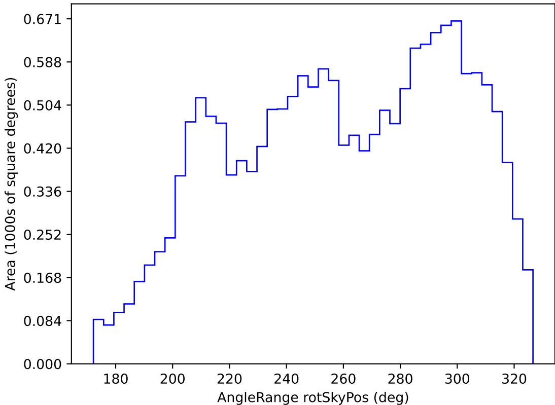
no_high_blob_v3.3_10yrs WFD u band: AngleRange rotSkyPos
