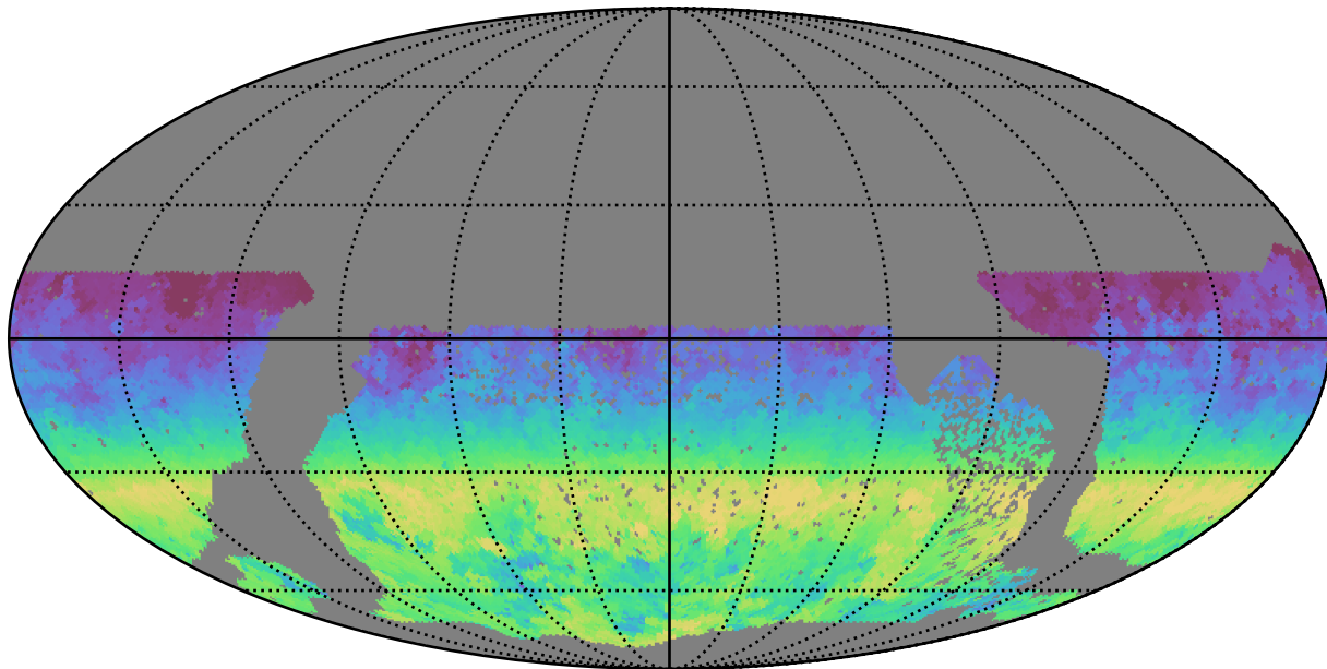
no_high_blob_v3.3_10yrs WFD i band: AngleRange rotSkyPos
