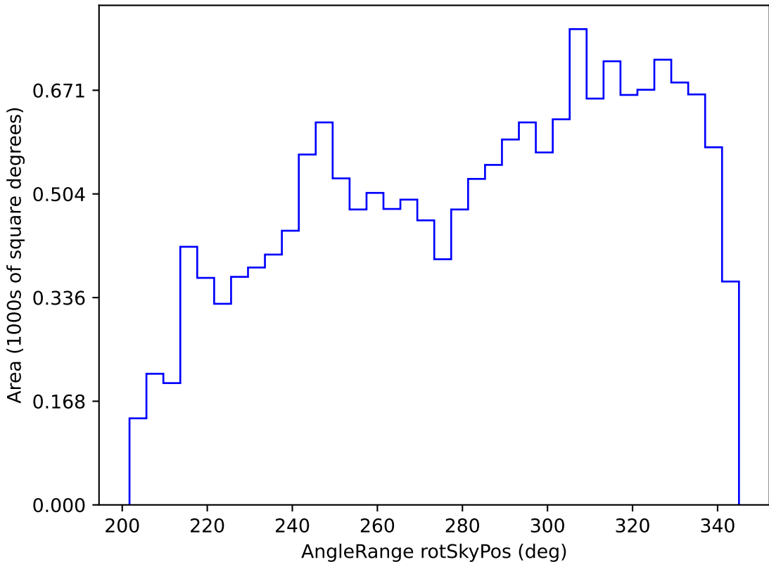
no_high_blob_v3.3_10yrs WFD i band: AngleRange rotSkyPos
