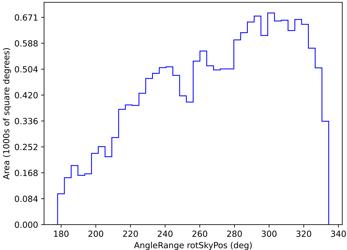
no_high_blob_v3.3_10yrs WFD g band: AngleRange rotSkyPos
