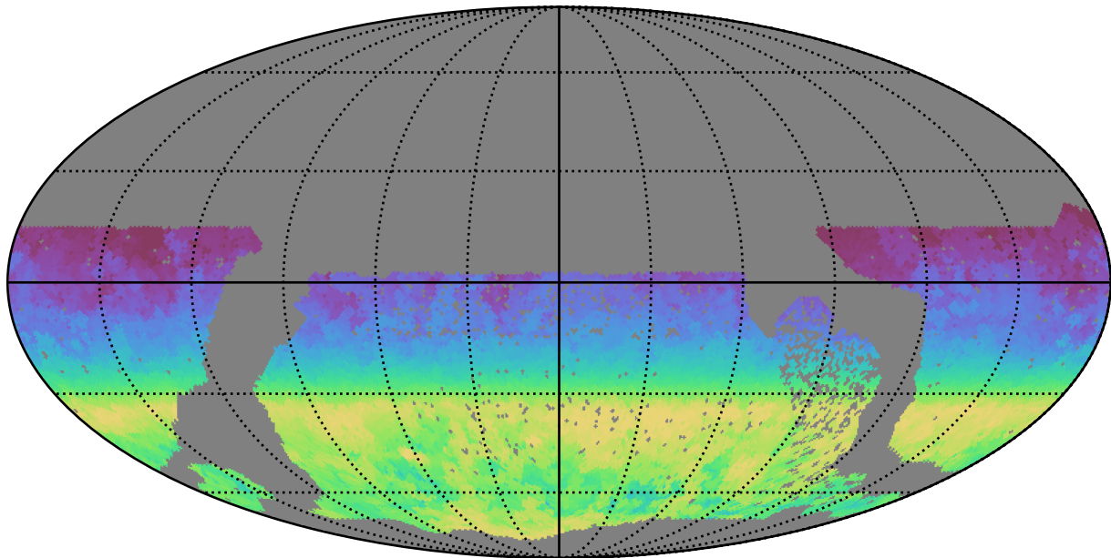
no_high_blob_v3.3_10yrs WFD all bands: AngleRange rotSkyPos
