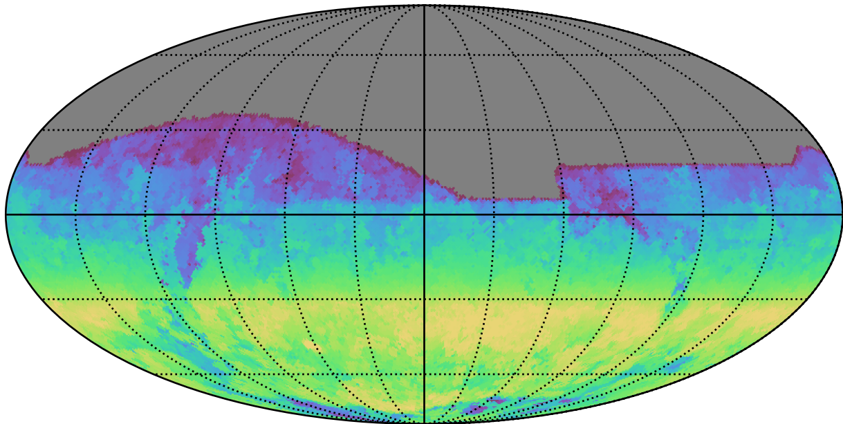
no_high_blob_v3.3_10yrs All sky z band: AngleRange rotSkyPos
