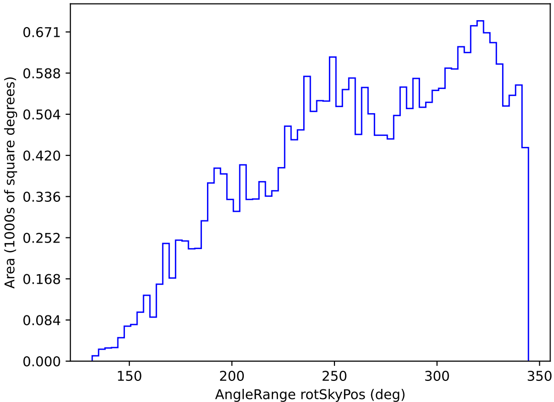
no_high_blob_v3.3_10yrs All sky z band: AngleRange rotSkyPos
