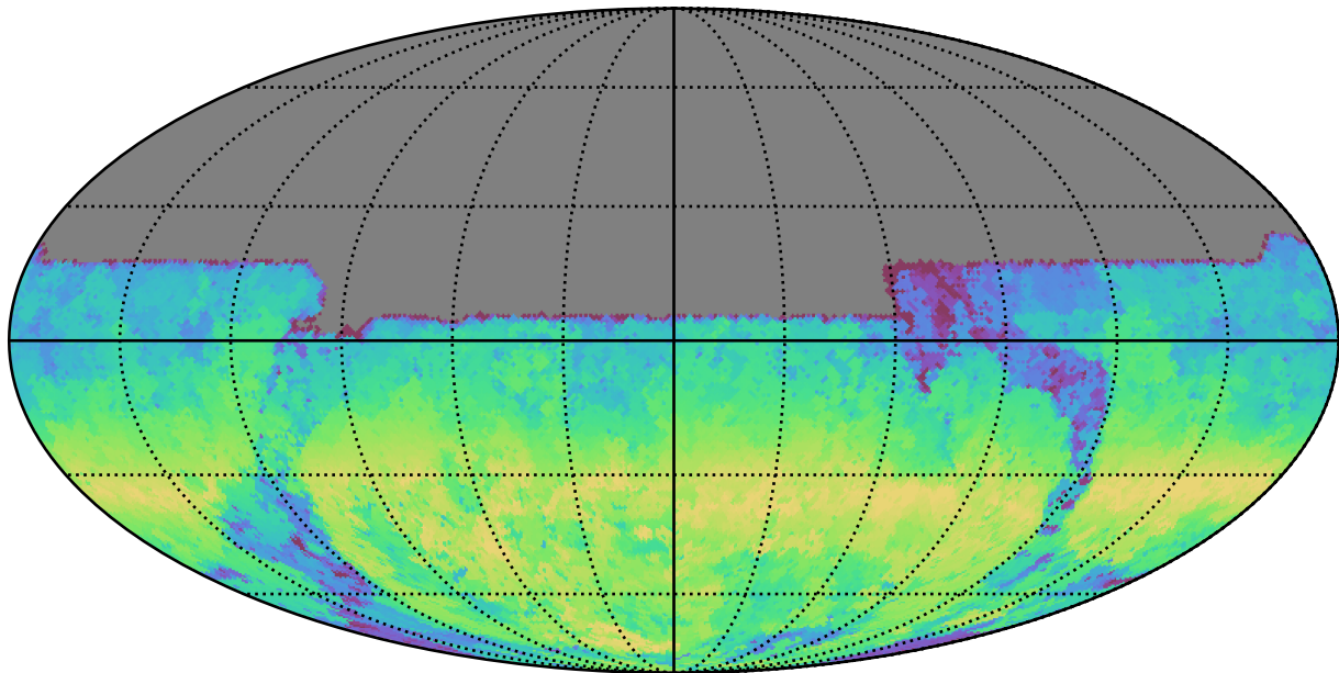
no_high_blob_v3.3_10yrs All sky u band: AngleRange rotSkyPos
