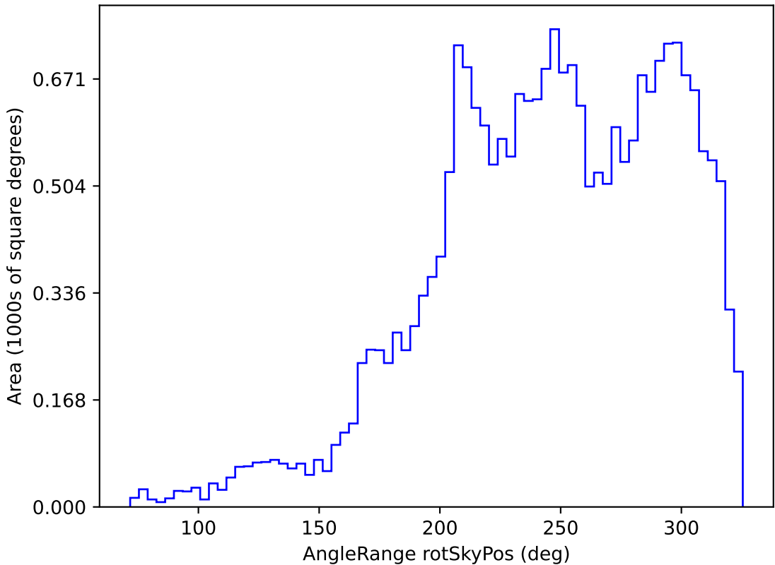
no_high_blob_v3.3_10yrs All sky u band: AngleRange rotSkyPos
