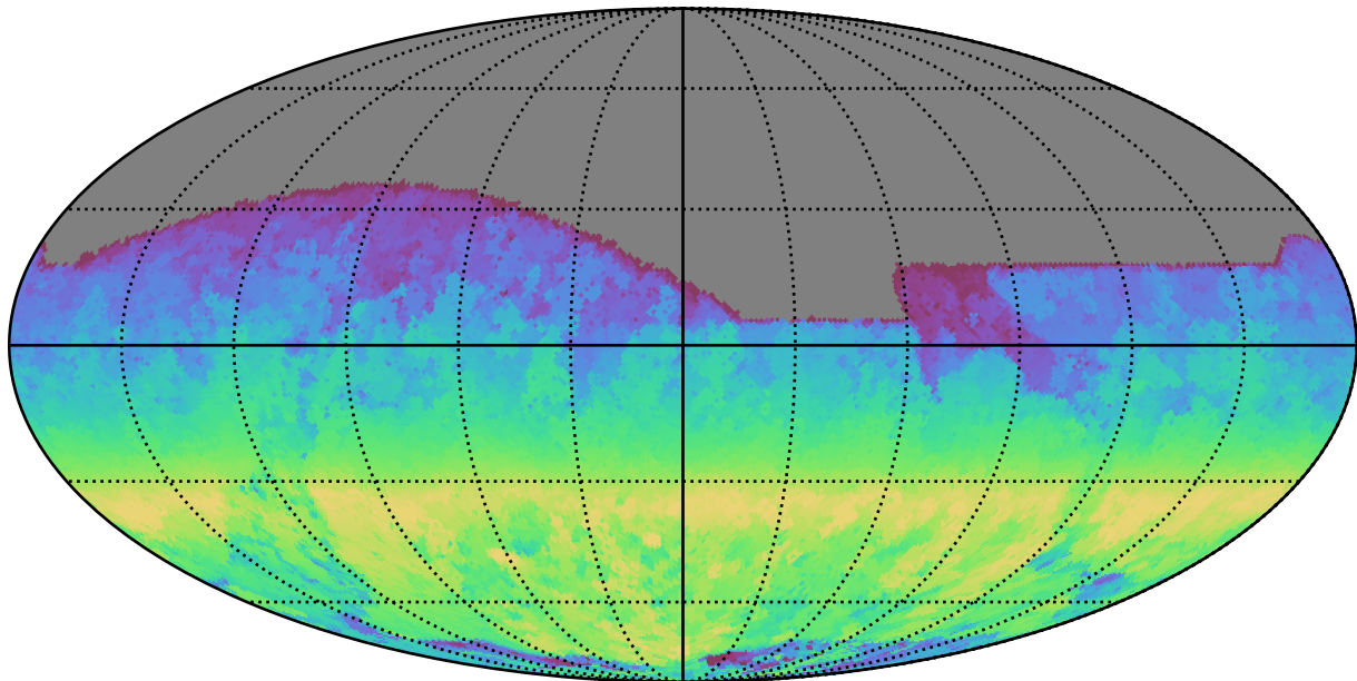
no_high_blob_v3.3_10yrs All sky r band: AngleRange rotSkyPos
