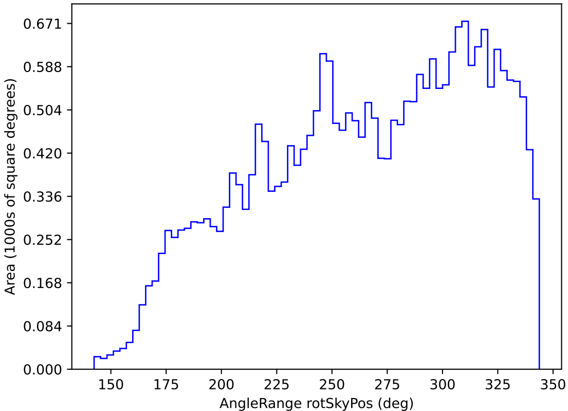
no_high_blob_v3.3_10yrs All sky i band: AngleRange rotSkyPos
