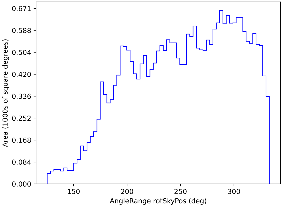
no_high_blob_v3.3_10yrs All sky g band: AngleRange rotSkyPos
