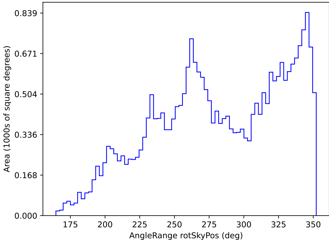
no_high_blob_v3.3_10yrs All sky all bands: AngleRange rotSkyPos
