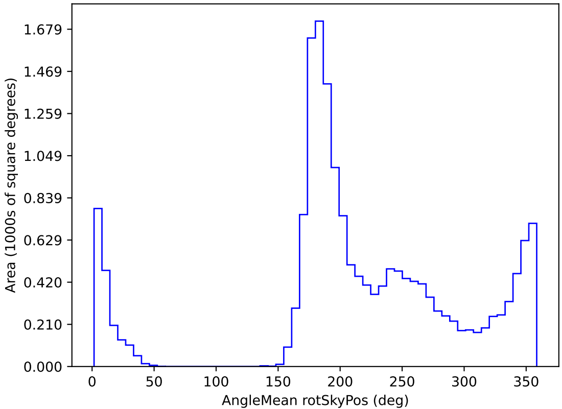
no_high_blob_v3.3_10yrs WFD z band: AngleMean rotSkyPos
