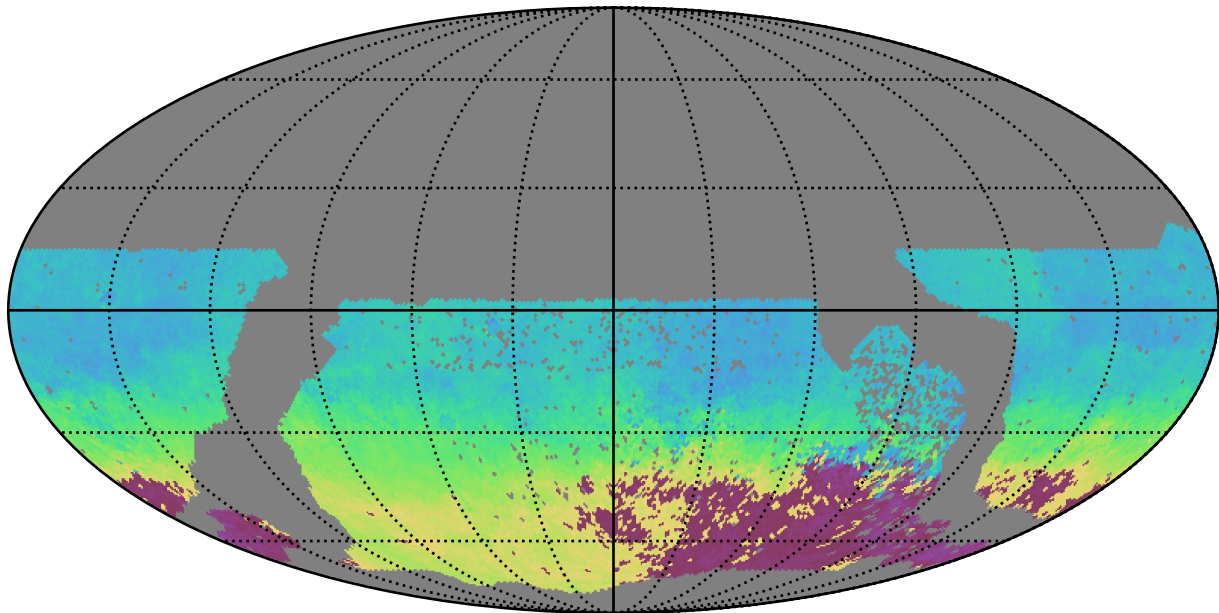
no_high_blob_v3.3_10yrs WFD u band: AngleMean rotSkyPos
