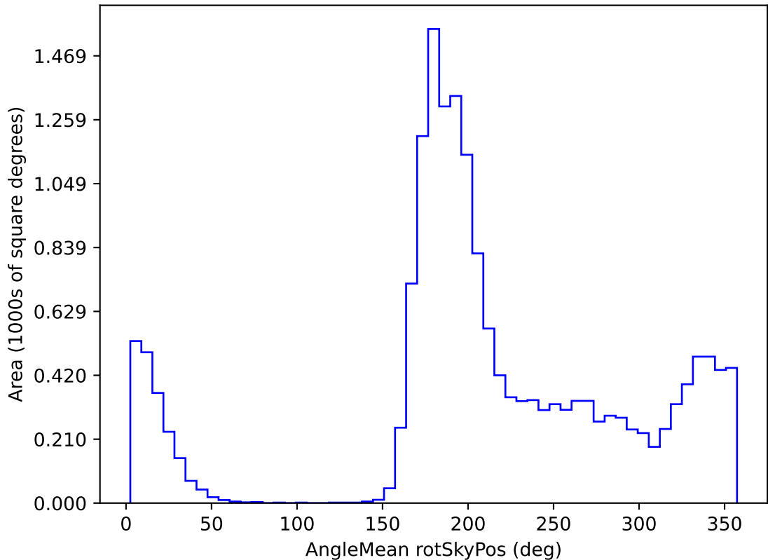
no_high_blob_v3.3_10yrs WFD u band: AngleMean rotSkyPos
